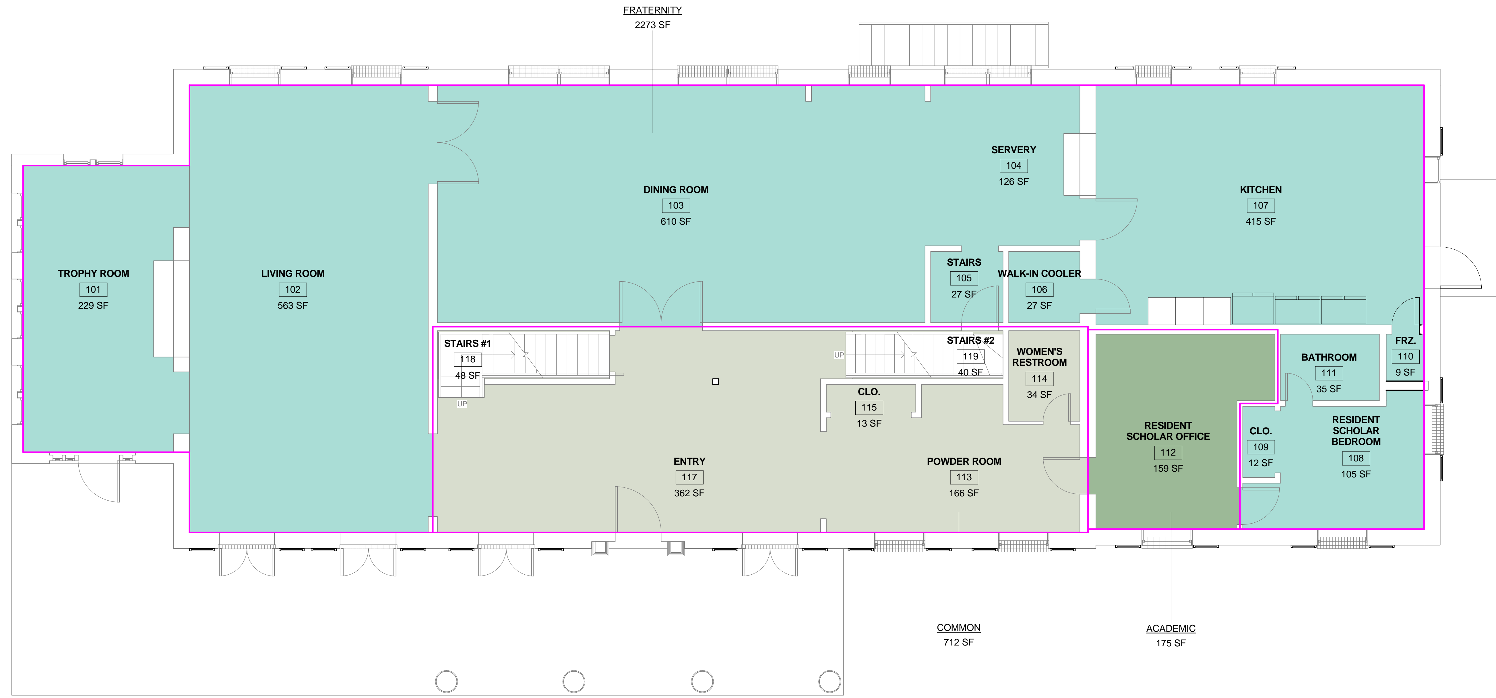
Room Schedule - CONSTRUCTION - LEVEL 1
